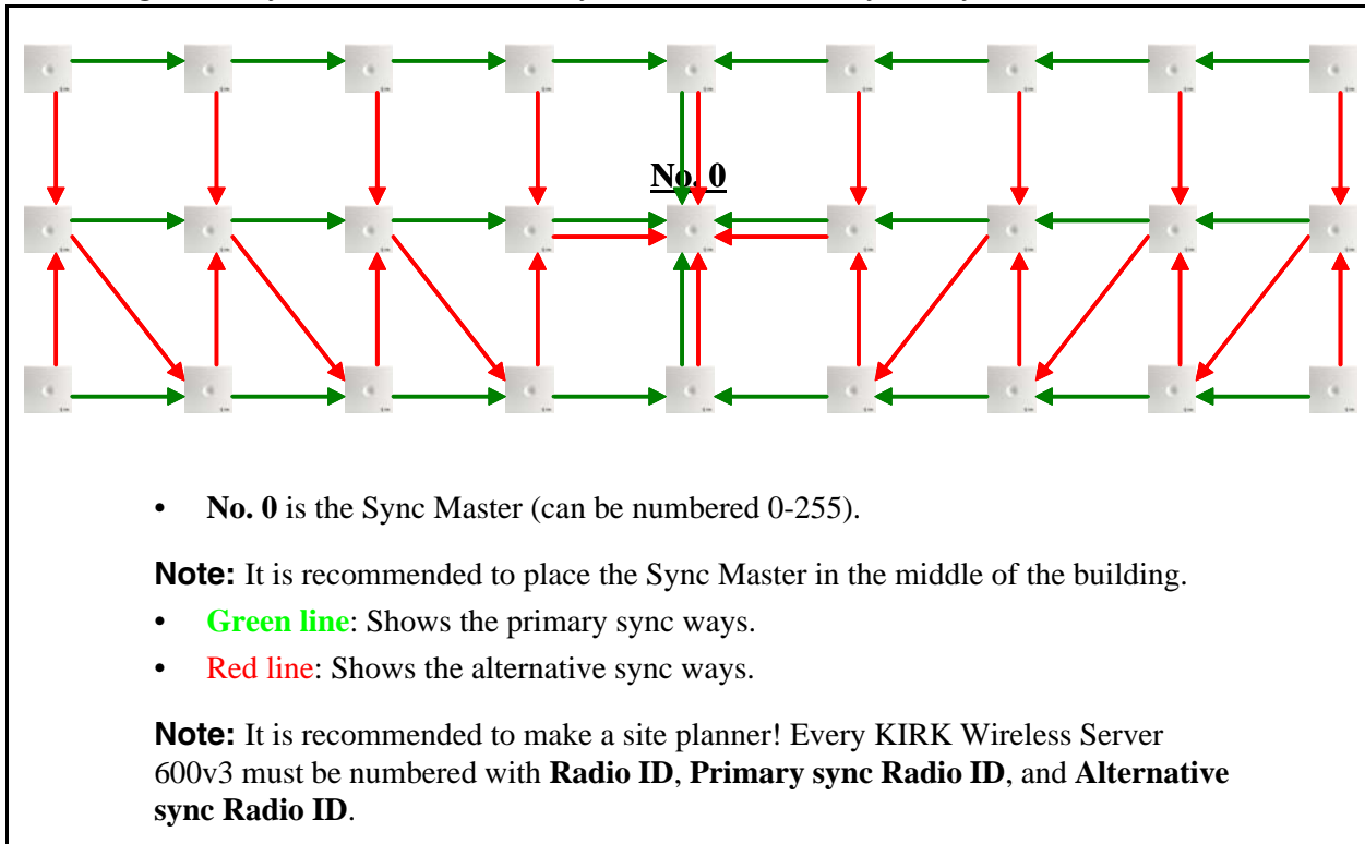
Figure 7 Synchronization Chain Layout with Alternative Sync Ways
